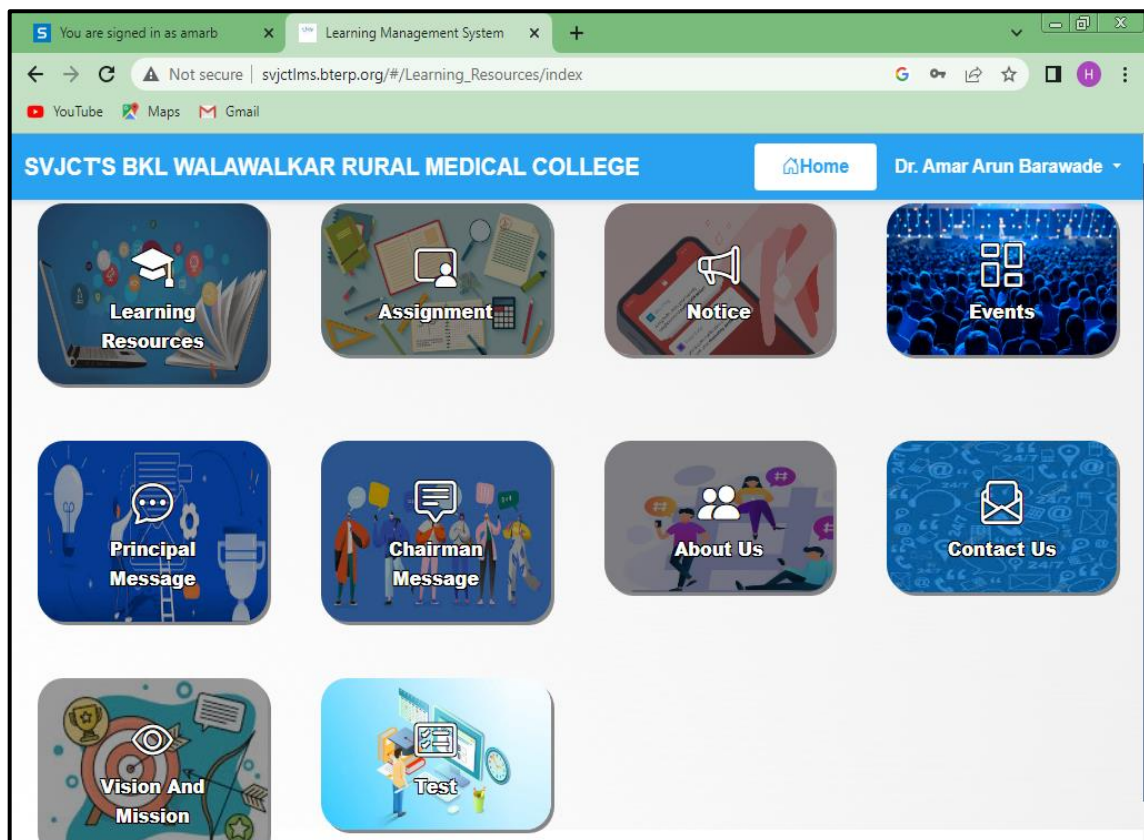
LMS Dashboard
